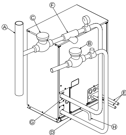
Heat source unit sample installation
